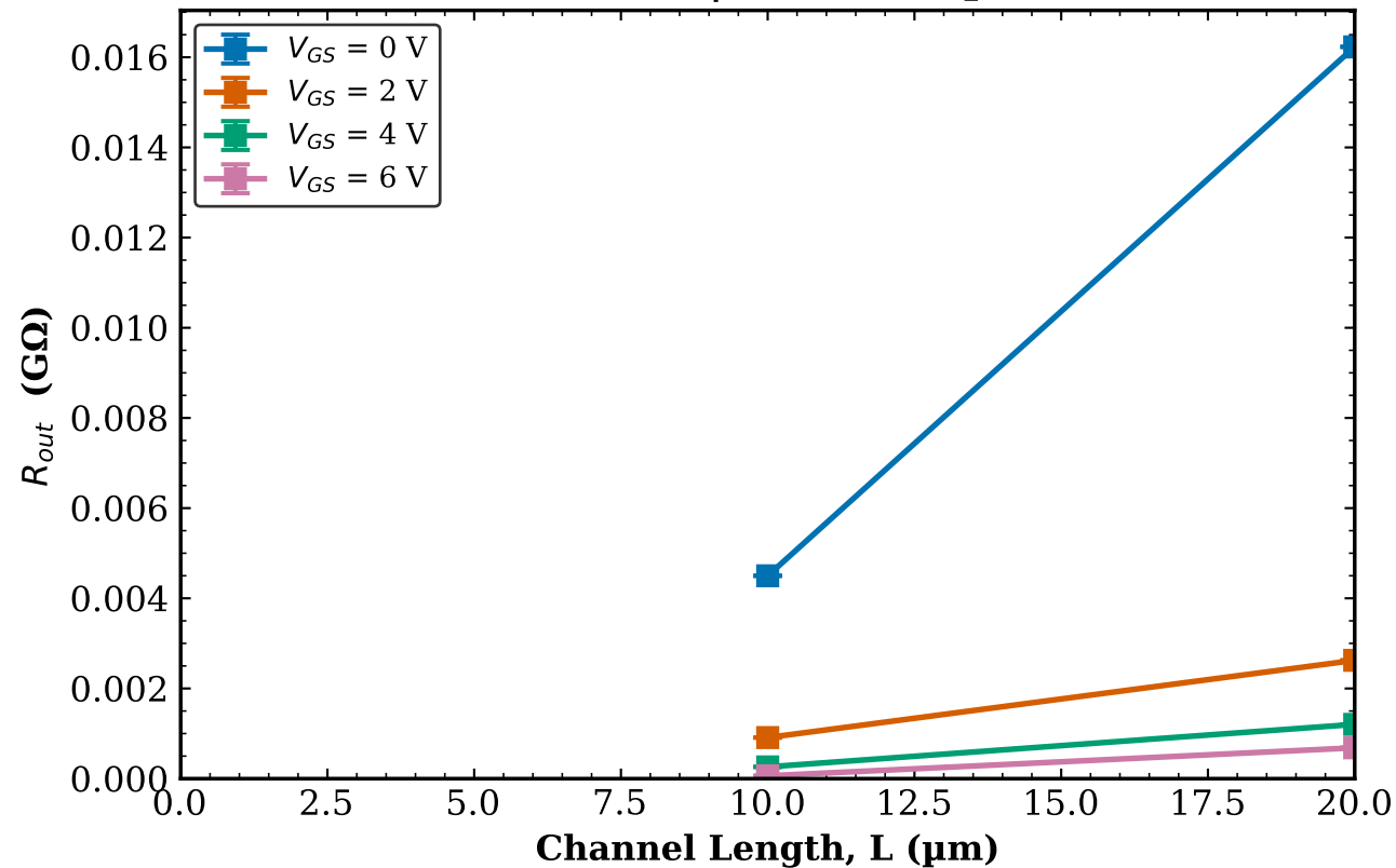
TFT1 Transistor 2 R_{out} vs L | W = 500\text{ }\mu\text{m}
